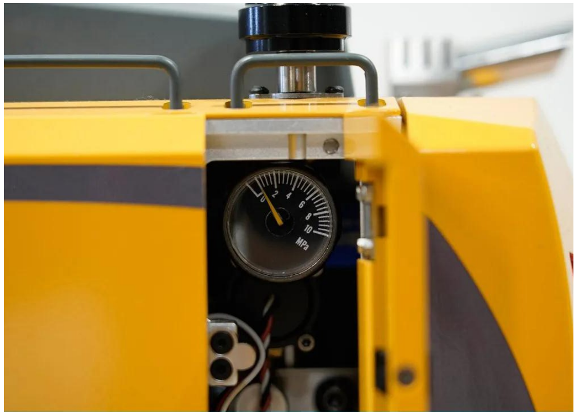
Instrument Warehouse Mechanical Pressure Gauge, Visual Display of Hydraulic Pressure
