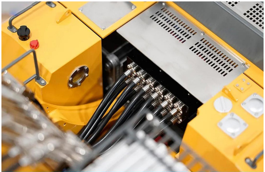
Integrated Multi-channel Hydraulic Pipeline Distributor
